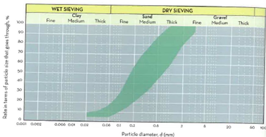
Fig. 8. Granulometry graph for mixtures in rooting layers.
